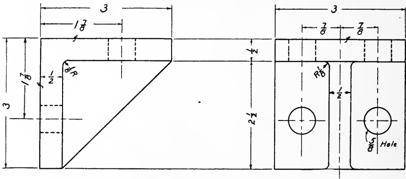
FIG. 522. MACHINIST'S DRAWING.
